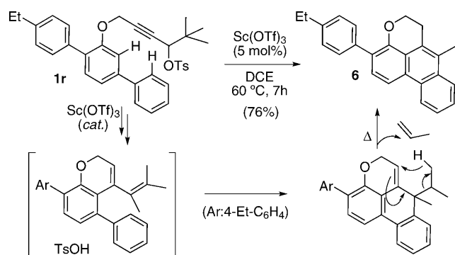
Scheme 6. Mechanistic interpretation for the formation of 6 .
