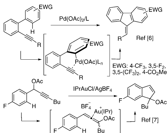
Scheme 1. Arene–alkyne cyclizations of electron-poor arene units. EWG = electron-withdrawing group.
