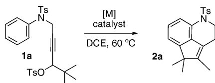
Scheme 3. Carbocyclization of 1a into 2a (see Table 1 for the reaction conditions).
