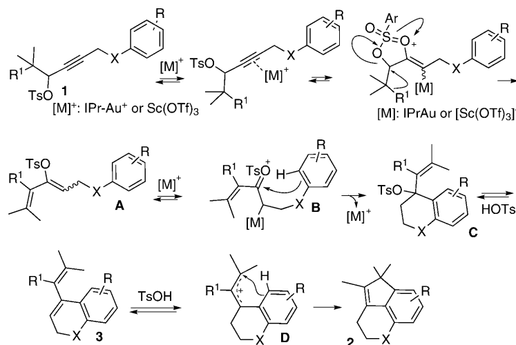
Scheme 5. Proposed working-model for the evolution of 1 into 2 .
