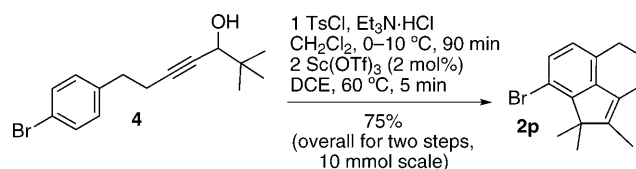
Scheme 4. C–H functionalization of ω-aryl-substituted propargylic alcohol derivatives: tosylation and double arylation reactions.
